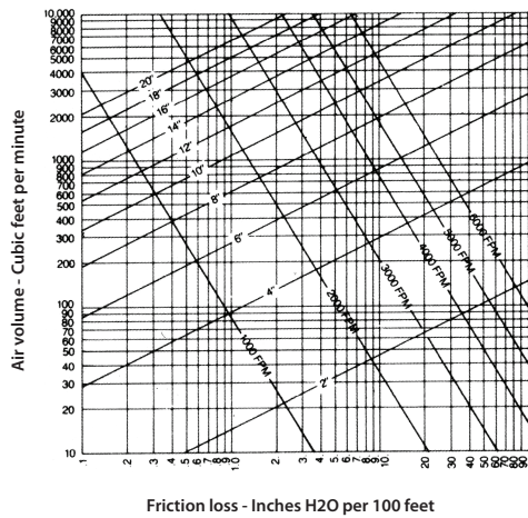
Flexible Duct - Straight Run Friction Loss per 100ft
