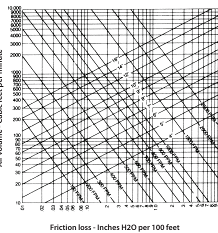
Flexible Duct - Straight Run Friction Loss per 100ft
